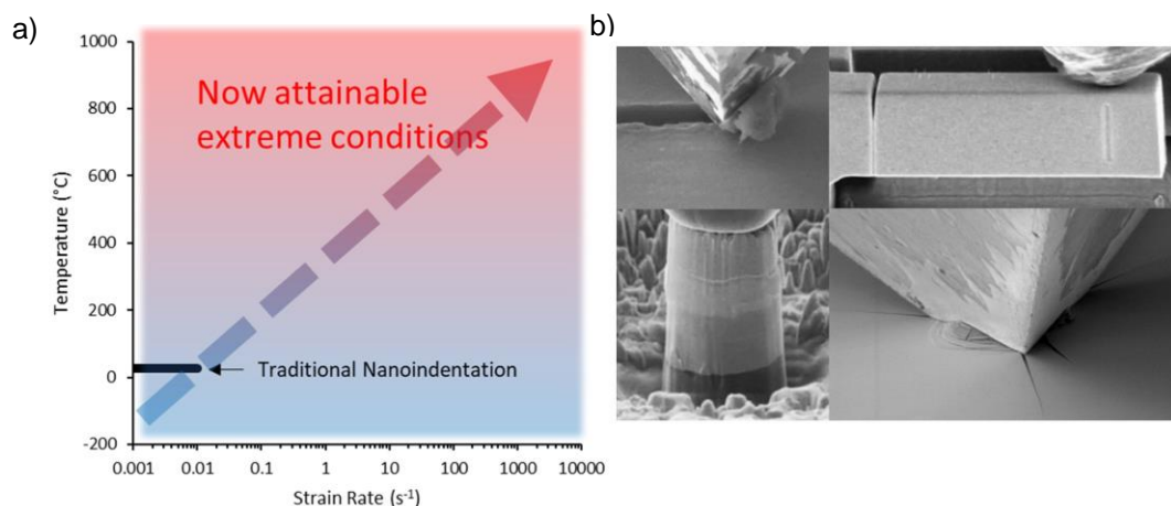
Figure 1 | a) Extreme conditions testing from low- to high temperatures at low- to high strain rates. b) overview of typical applications and test geometries of in situ micromechanical testing.
